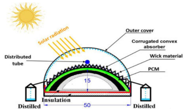
Fig. 1. Schematic diagram of tubular solar still with v-corrugated absorber.
