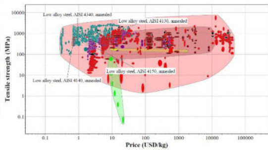
Figure 4, Ashby Plot: Tensile Strength vs. Cost.
