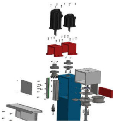
Figure 5, Exploded View of the Machine.
