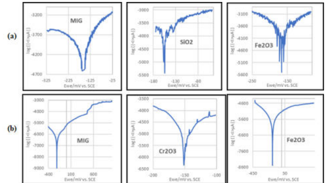
metals, and MIG and AMIG samples were welded with ER 308 L filler metal. (b) Potentiodynamic polarization graphs obtained for base metals MIG and AMIG samples welded with mild steel filler metal
