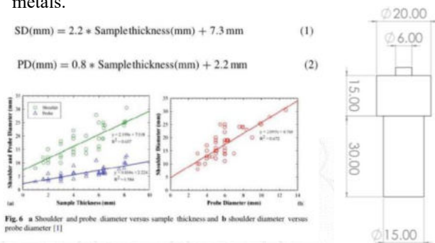
Figure 6, FSSW Tool Optimized Based on Research Findings.
